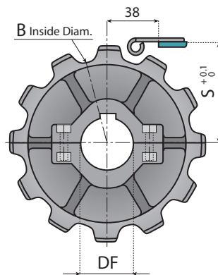
SPLIT SPROCKETS - Fixed
