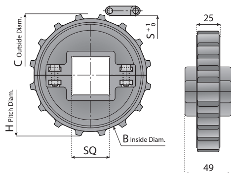
SPLIT SPROCKETS SQUARE BORE - Floating
