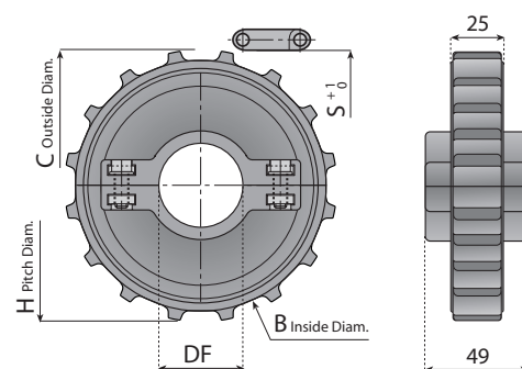
SPLIT IDLER WHEELS - Floating
