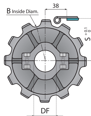
SPLIT IDLER WHEELS - Floating
