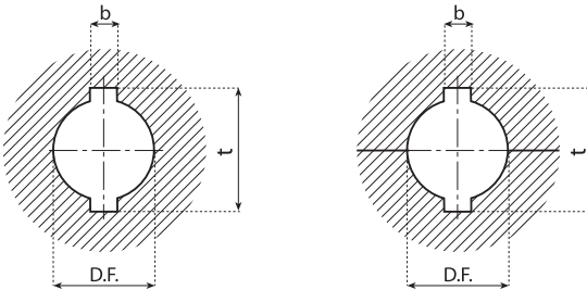
KEY TO BE USED ACCORDING TO UNI 6604 - 69 /ISO 773 - DIN 6885
