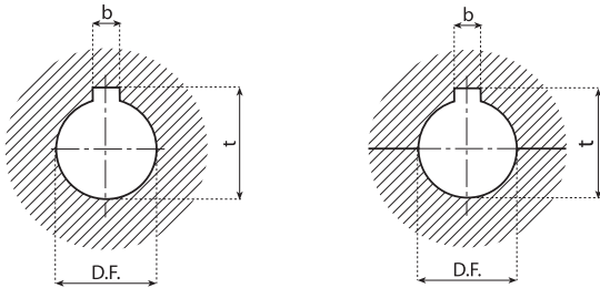
KEY TO BE USED ACCORDING TO UNI 6604 - 69 /ISO 773 - DIN 6885
