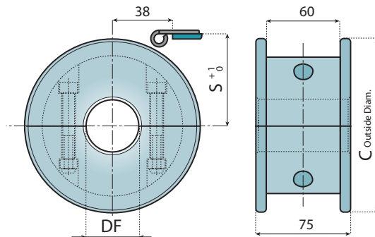
SPLIT IDLER WHEELS - Floating
