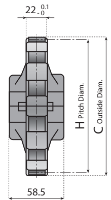
SPLIT IDLER WHEELS - Floating
