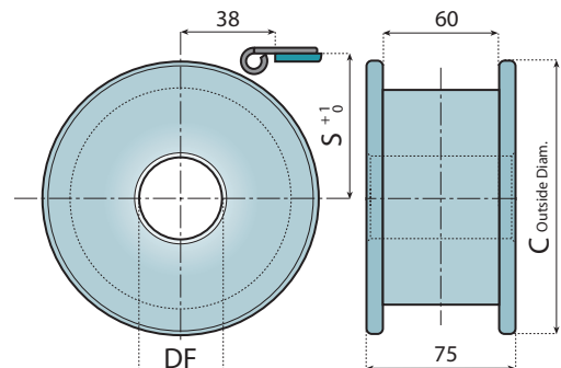
ONE PIECE IDLER WHEELS - Floating
